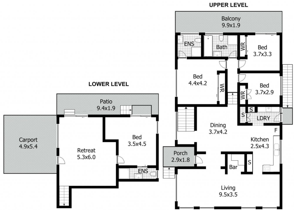
FLOOR PLAN
