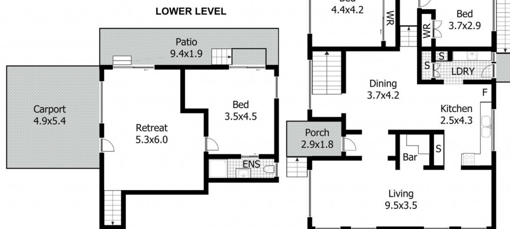
FLOOR PLAN
